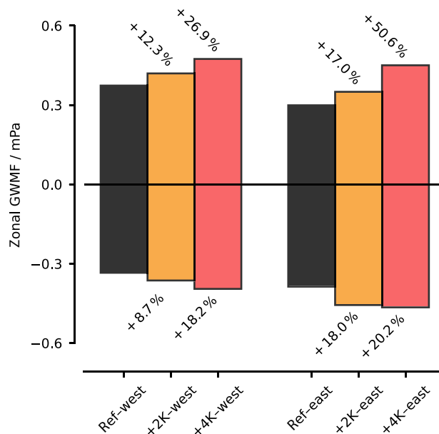
FIGURE 6 Zonal mean zonal gravity wave momentum flux (GWMF; i.e., vertical flux of zonal wave momentum) at an altitude of 20 km averaged over 15^\circ S– 15^\circ N for the last 30 simulation days. Positive bars show eastward GWMF and negative bars show westward GWMF. Annotations show the increase in eastward and westward GWMF of the warmer climate states relative to their corresponding reference climate. The zonal GWMF has been calculated by means of the small-volume few-wave decomposition (S3D; see Section 2.4.2). [Colour figure can be viewed at wileyonlinelibrary.com ]
