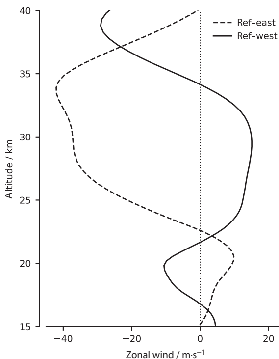
FIGURE 1 The 5° S – 5° N zonal mean zonal wind profiles in the stratosphere at model initialization.
