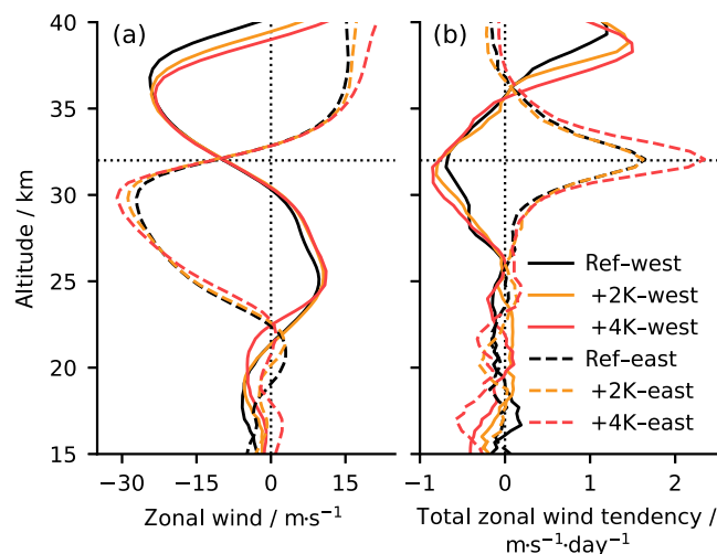
FIGURE 9 The 5^{\circ}\text{S} – 5^{\circ}\text{N} mean QBO composites of the 11-day period during which the zonal mean zonal wind profiles cross the -10 \text{ m s}^{-1} -wind line closest at a reference height of 32 km: (a) zonal wind and (b) total zonal wind tendency. The reference height is marked by the horizontal dotted black line. [Colour figure can be viewed at wileyonlinelibrary.com ]
